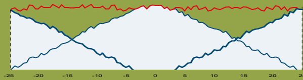
Working width: 28 m at 250 Kg/ha
