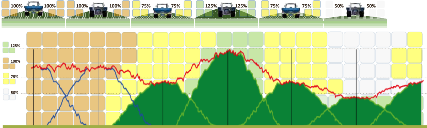
Flexibility at highest level Differential application from 150 Kg/ha to 450 Kg/ha at 28 meter.
